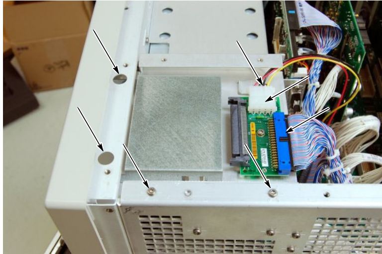
Figure 13: Removing cables from the IDE adapter board and removing the screws that secure assembly
