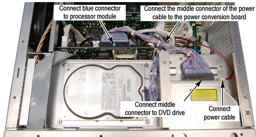
Figure 20: Connecting IDE cable and power cable to the DVD-R/W drive
